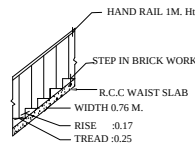
STAIR DETAIL
