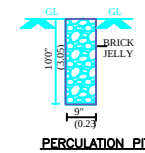
PERCOLATION PIT
