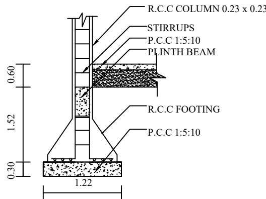
COLUMN DETAILS
