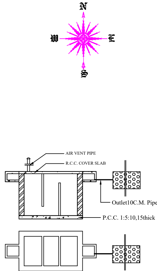
Septic Tank and Trench
