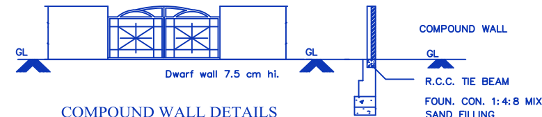
COMPOUND WALL DETAILS
