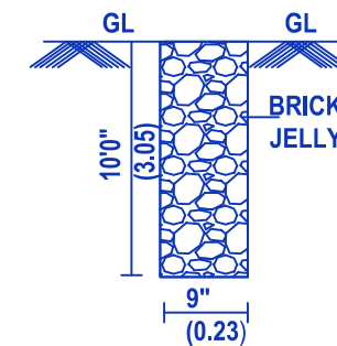
PERCULATION PIT
