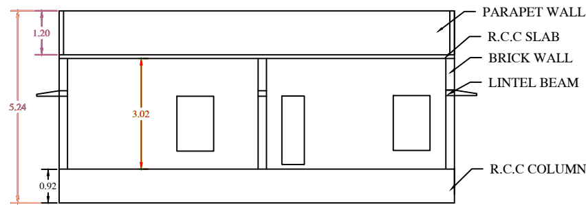
SECTION AT X-X'
