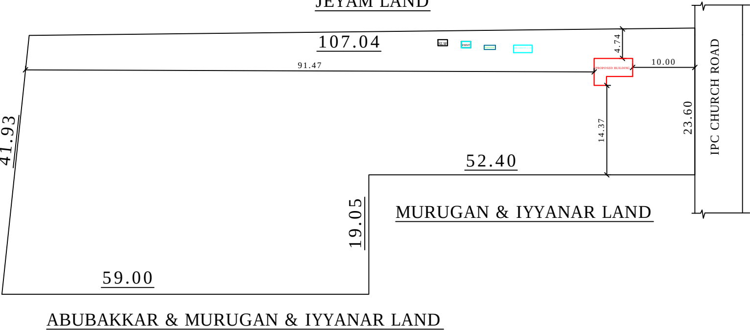
SITE PLAN
