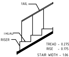
STAIRCASE DETAILS NTS
