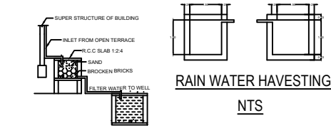
DETAILS OF FILTER BED & WELL NTS
