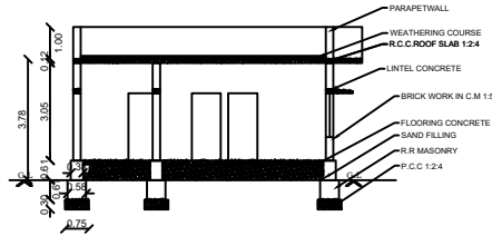
SECTION AT A-B
