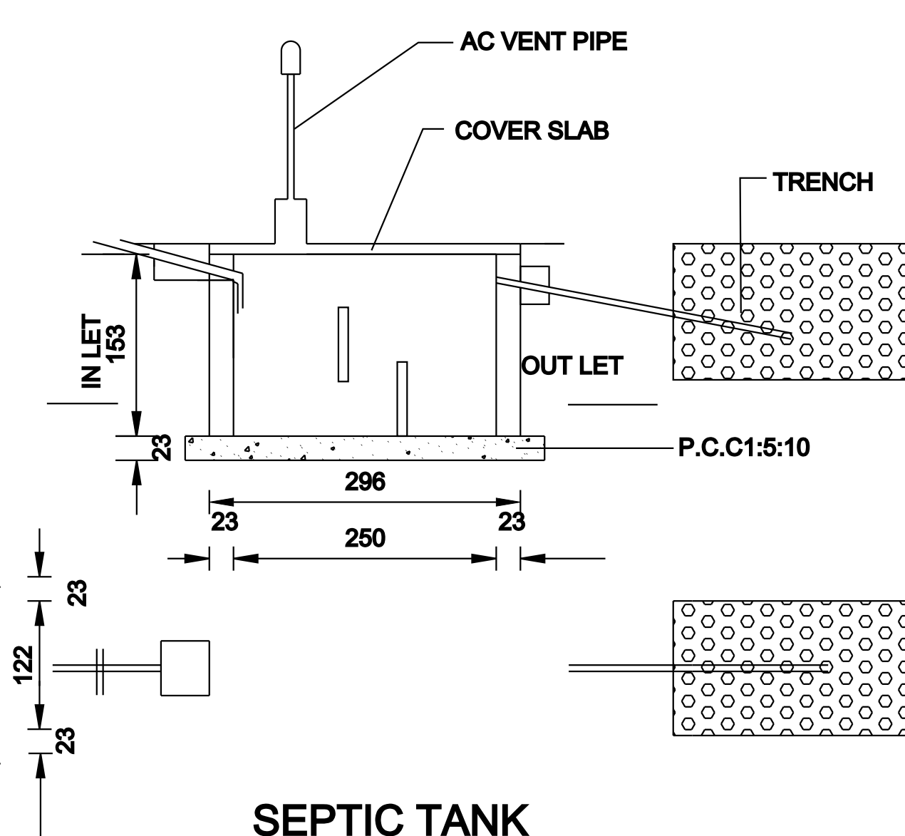
SEPTIC TANK
