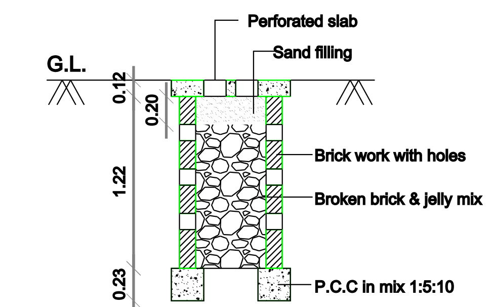
PERCOLATION PIT FOR 30 Sq. m.
