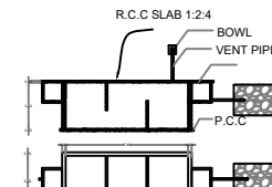
SEPTIC TANK AND TRENCH NTS
