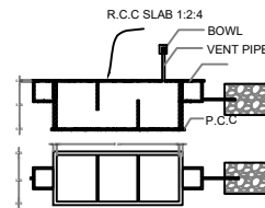
SEPTIC TANK AND TRENCH NTS
