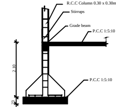
Column Detail
