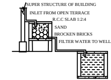
Rainwater harvesting
