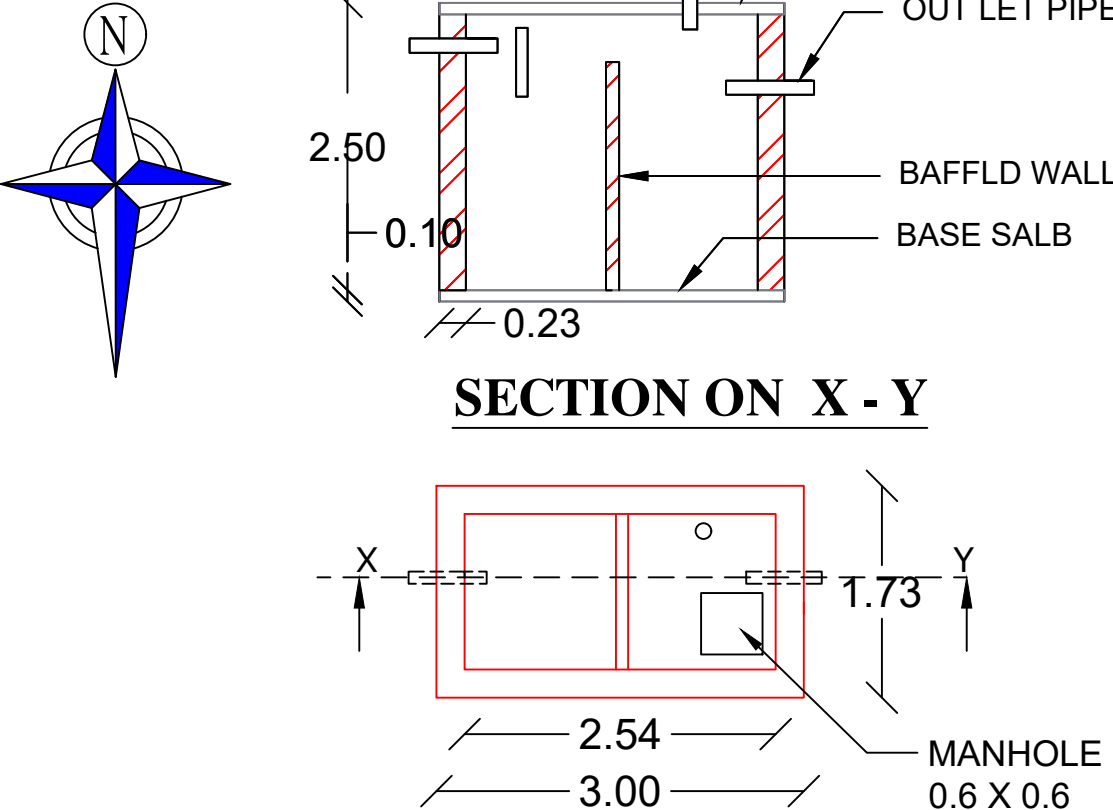
SEPTIC TANK PLAN
