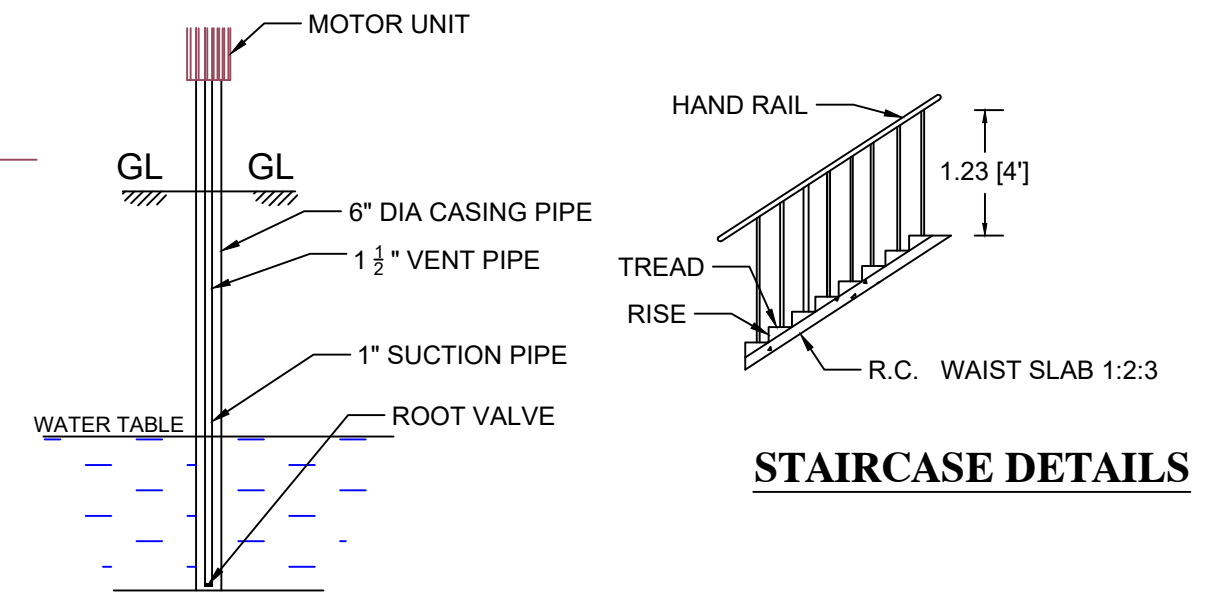
SEC.OF BOREWELL
