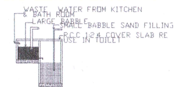
RECYCLING OF WASTE WATER FROM KITCHEN & BATHROOM
