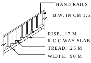
SECTION ON STAIR
