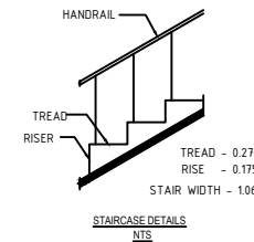
STAIRCASE DETAILS NTS
