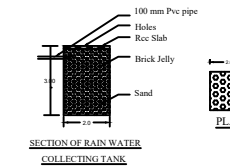
SECTION OF RAIN WATER COLLECTING TANK
