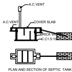
PLAN AND SECTION OF SEPTIC TANK
