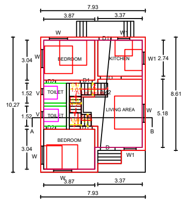
GROND FLOOR PLAN
