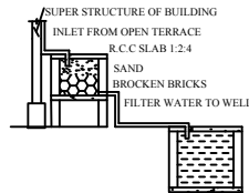
Rainwater harvesting
