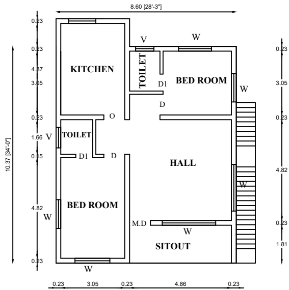
REV. FIRST FLOOR PLAN
