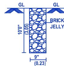
PERCOLATION PIT
