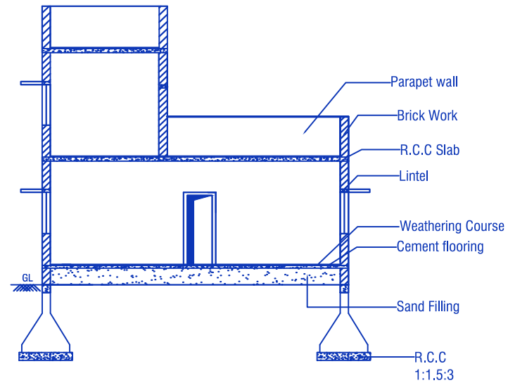
CROSS SECTION ON 'AB'
