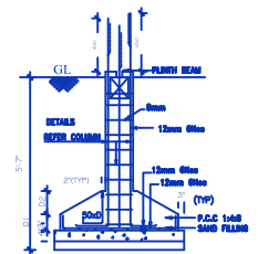
FOUNDATION DETAILS
