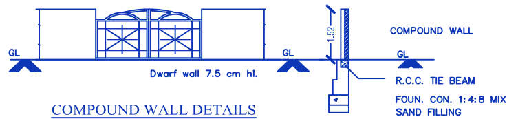
COMPOUND WALL DETAILS
