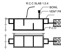
SEPTIC TANK AND TRENCH
