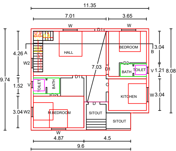
GROND FLOOR PLAN
