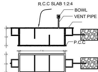
SEPTIC TANK AND TRENCH NTS
