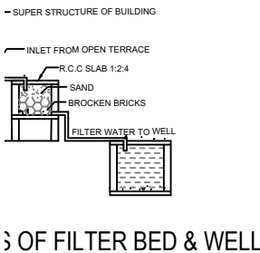
SECTION OF FILTER BED & WELL NTS
