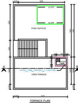
TERRACE PLAN
