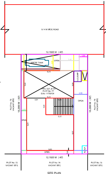
SITE PLAN
