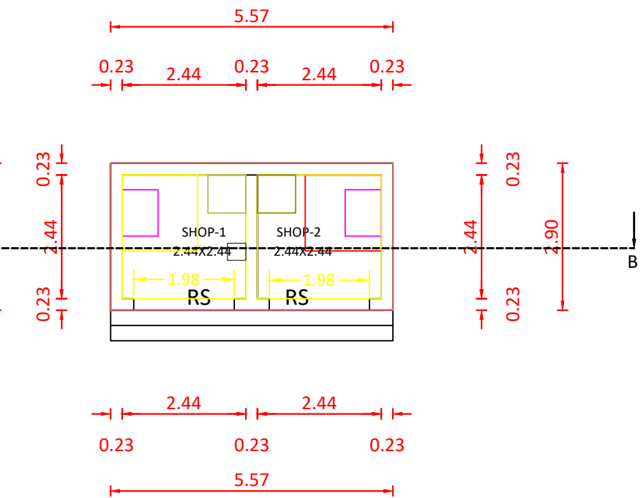
BLOCK-1-GROUND FLOOR SHOP PLAN
