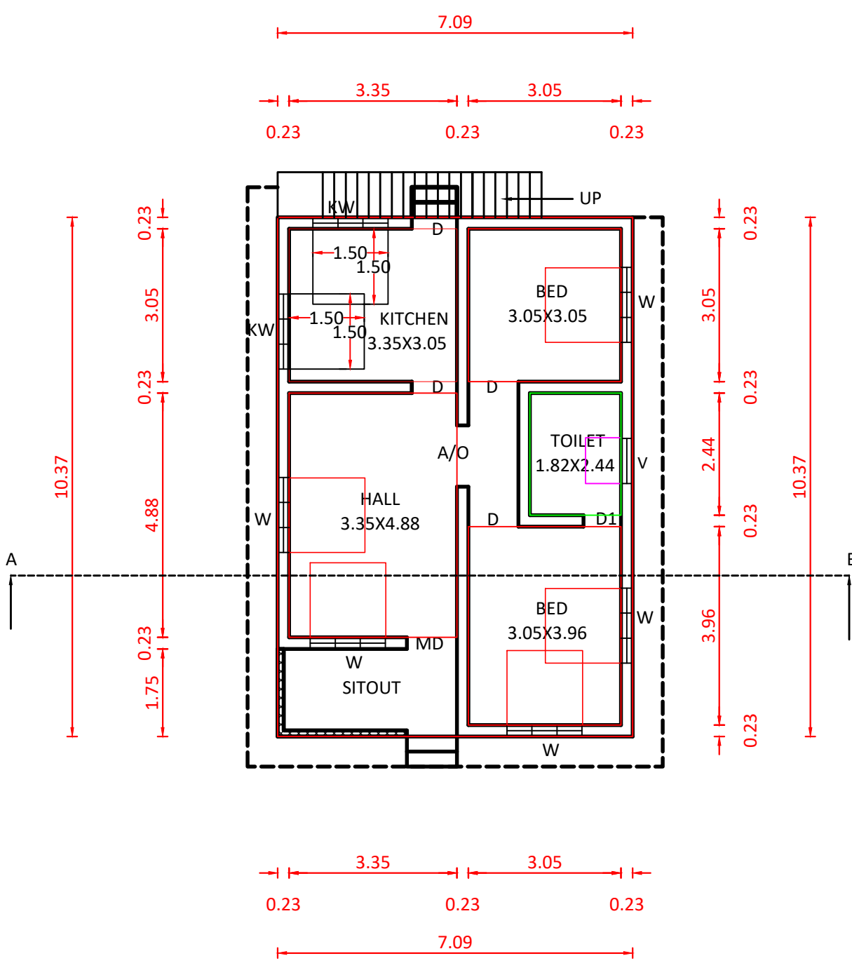
BLOCK-2-GROUND FLOOR HOUSE PLAN
