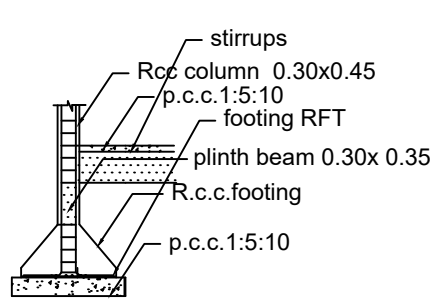
COLUMN DETAILS
