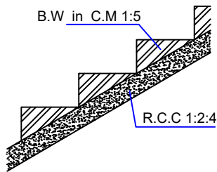
STAIRCASE
