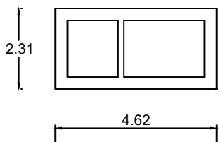
PLAN SEPTIC TANK DETAILS
