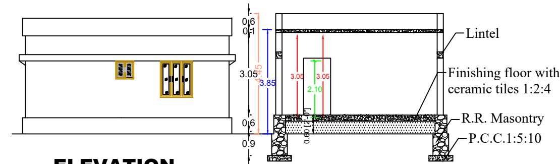
SECTION AB
