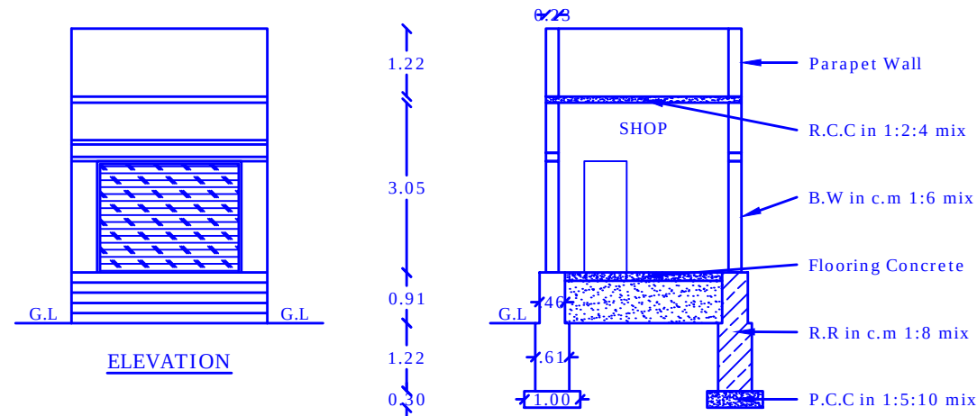
CROSS SECTION
