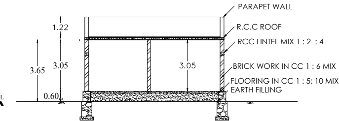
SECTION ON AB & ( HALF ELEVATION)
