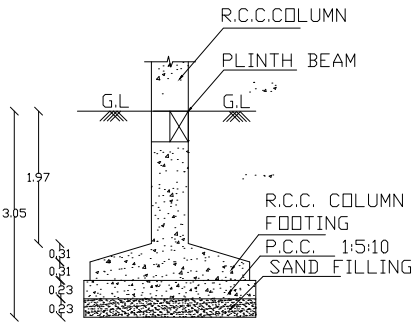
FOUNDATION DETAIL
