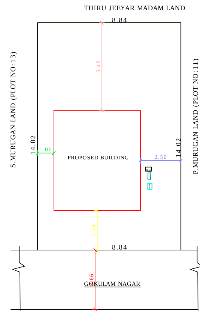
SITE PLAN
