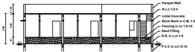
SECTION ON "AA"
