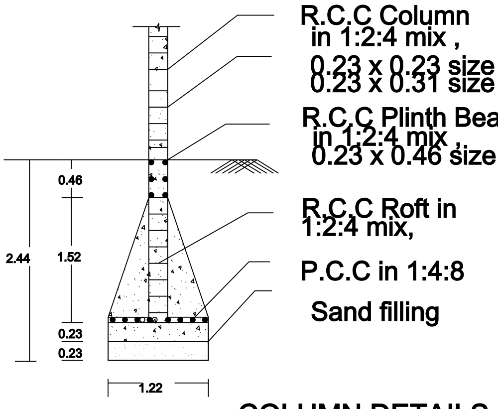
COLUMN DETAILS
