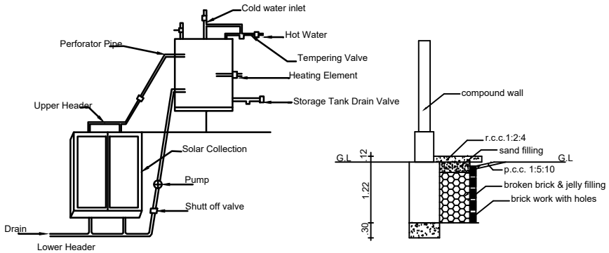
Details Of Solar Water Heater (NTS)
