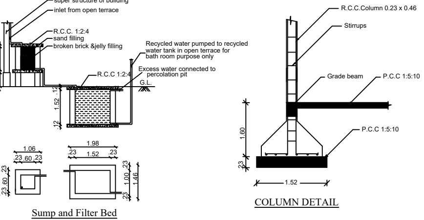
Sump and Filter Bed
