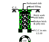
PERCOLATION PIT (NOT FOR SCALE)
