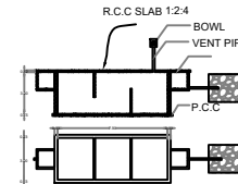
SEPTIC TANK AND TRENCH
