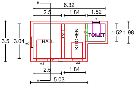
GROND FLOOR PLAN
