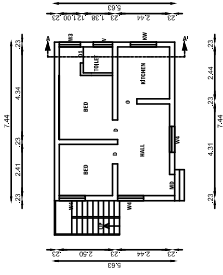
PRO. GROUND FLOOR (BLOCK 2) PLAN
