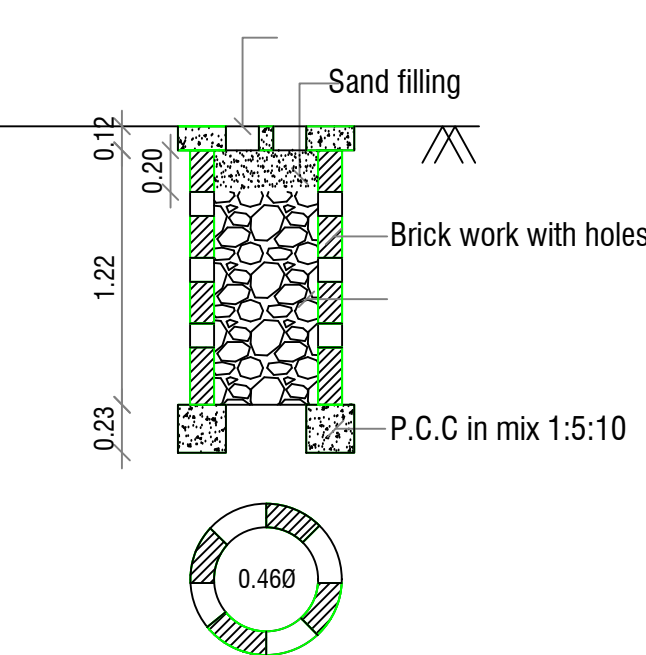
PERCOLATION PIT FOR 30 Sq. m.
