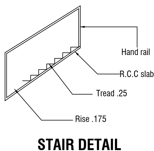
STAIR DETAIL
