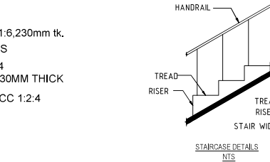
STAIRCASE DETAILS
