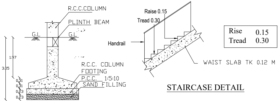
FOUNDATION DETAIL
