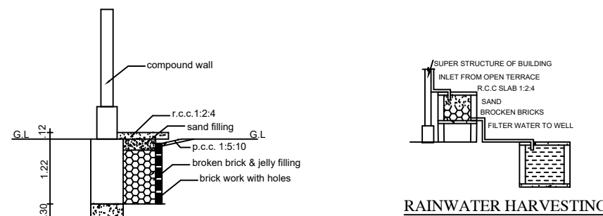
PLINTH BOUNDARY PERCOLATION PIT
