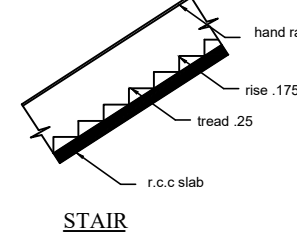
STAIR
