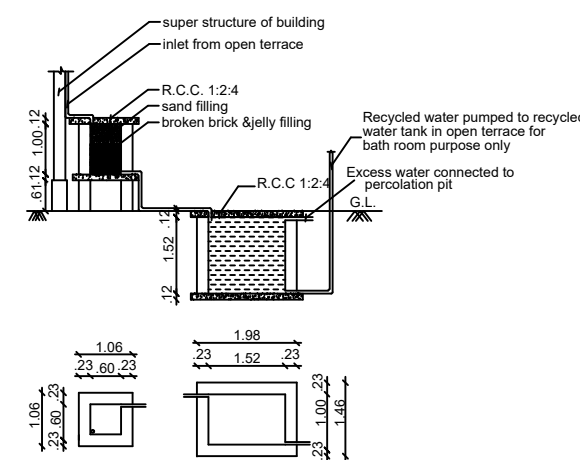
Sump and Filter Bed
