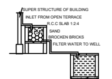
RAINWATER HARVESTING
