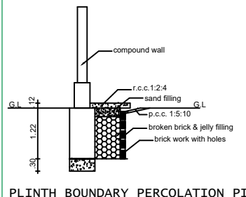
PLINTH BOUNDARY PERCOLATION PIT
