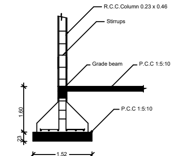
COLUMN DETAIL
