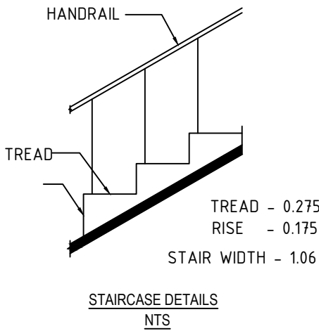
STAIRCASE DETAILS NTS
