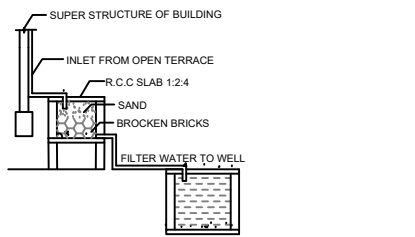
DETAILS OF FILTER BED & WELL NTS
