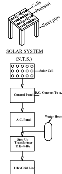
SOLAR SYSTEM FLOW DIAGRAM
