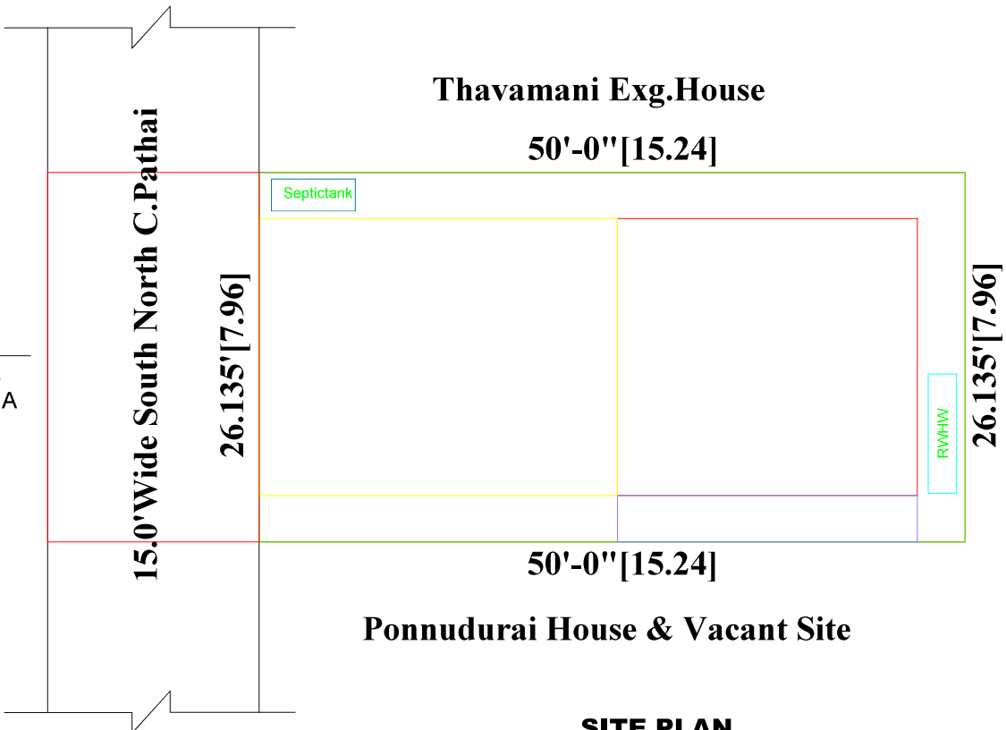
SITE PLAN
