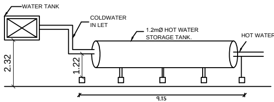
SOLAR WATER HEATING SWHS DETAIL
