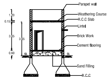
CROSS SECTION ON 'AB'
