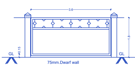
COMPOUND WALL/ ENTRANCE GATE
