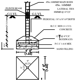
FOUNDATION DETAIL
