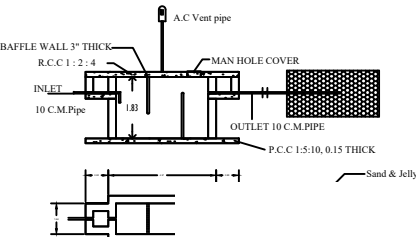
SEPTIC TANK
