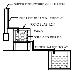
LS OF FILTER BED & WELL
