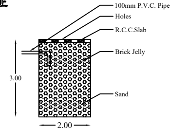
SECTION OF RAIN WATER COLLECTING TANK
